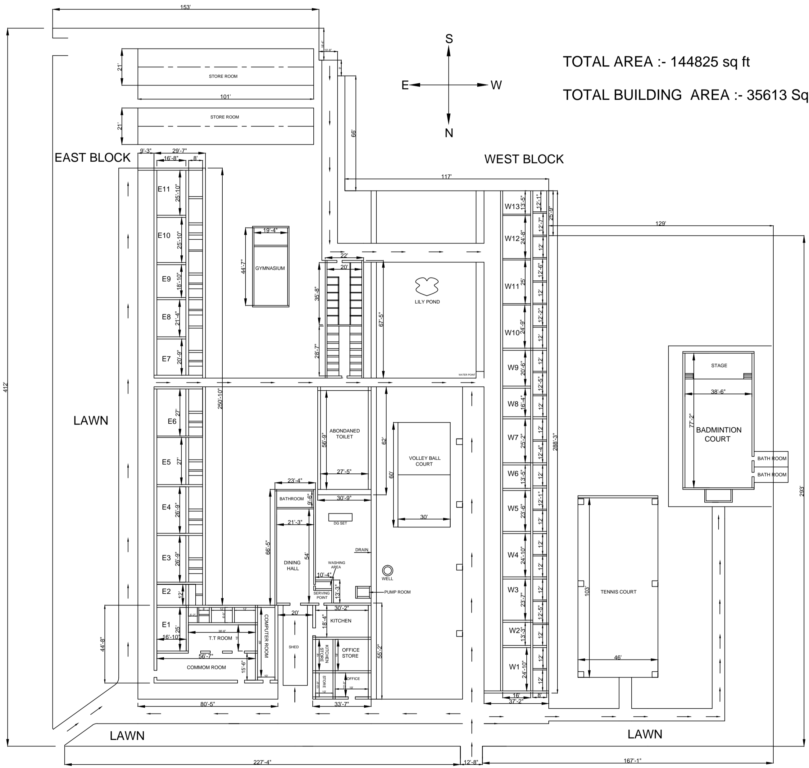
LAYOUT OF QUEENS ROAD HOSTEL(GROUND FLOOR)
